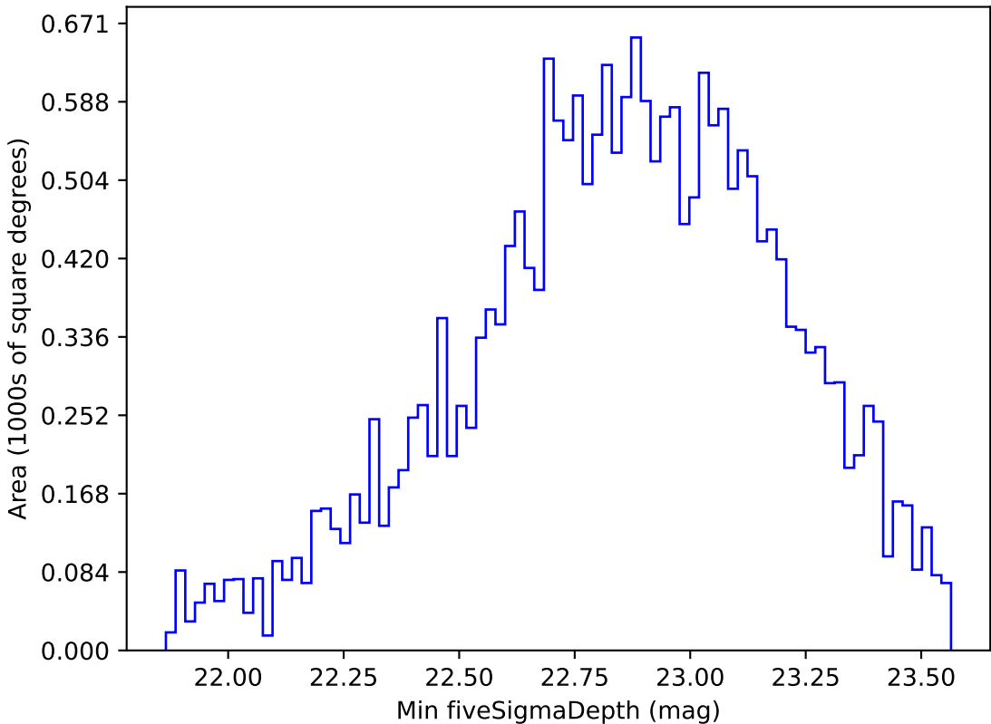
ddf_loaded_fl4_v3.4_10yrs Yr 1 u band: Min fiveSigmaDepth
