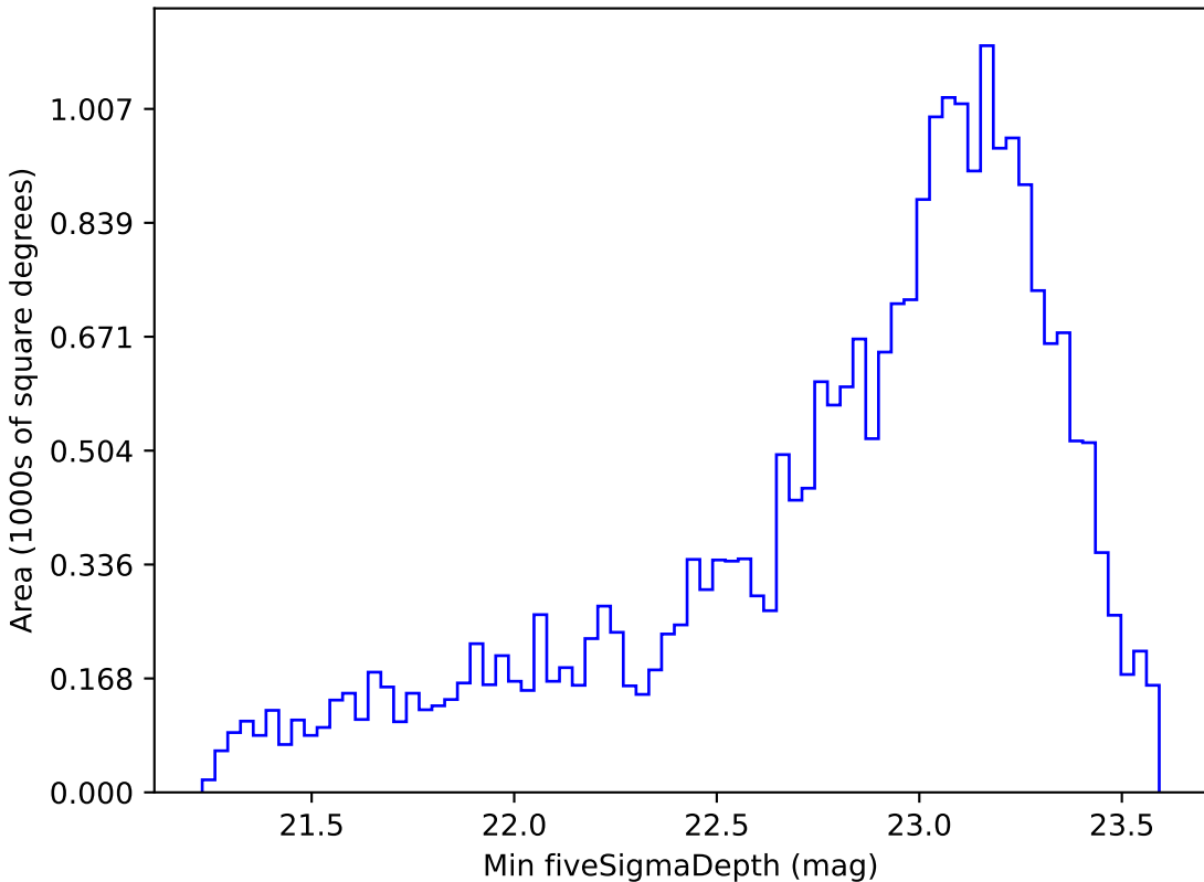
ddf_loaded_fl4_v3.4_10yrs Yr 1 i band: Min fiveSigmaDepth
