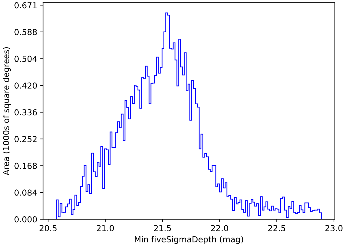
ddf_loaded_fl4_v3.4_10yrs Yr 1 all bands: Min fiveSigmaDepth
