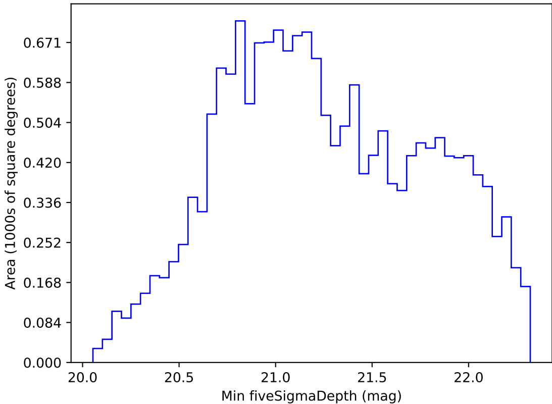
ddf_loaded_fl4_v3.4_10yrs WFD z band: Min fiveSigmaDepth
