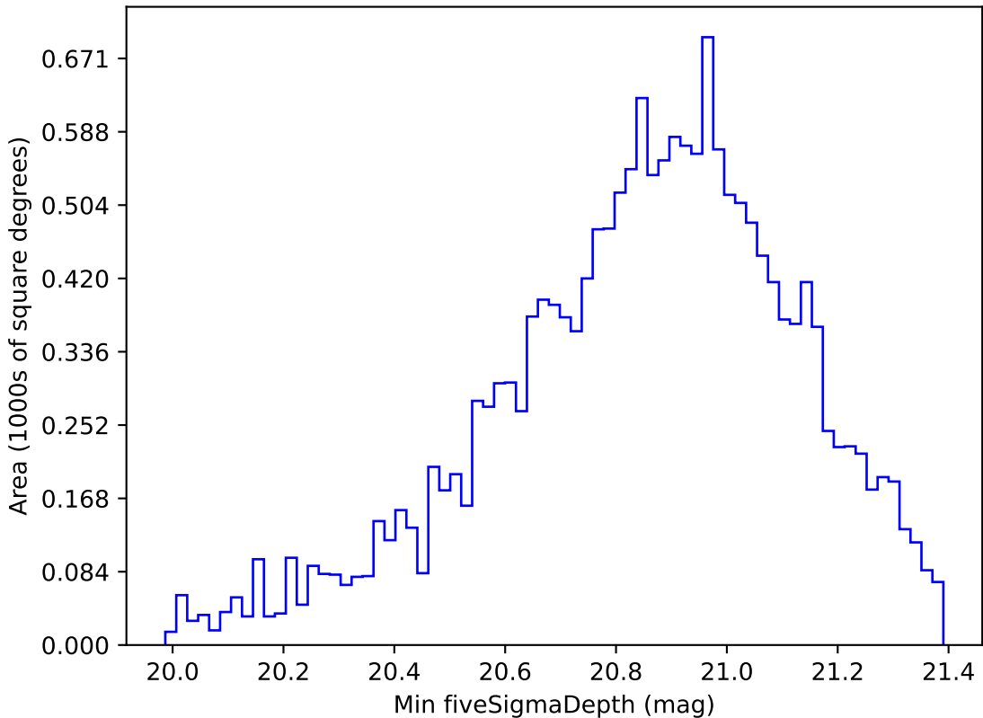
ddf_loaded_fl4_v3.4_10yrs WFD y band: Min fiveSigmaDepth
