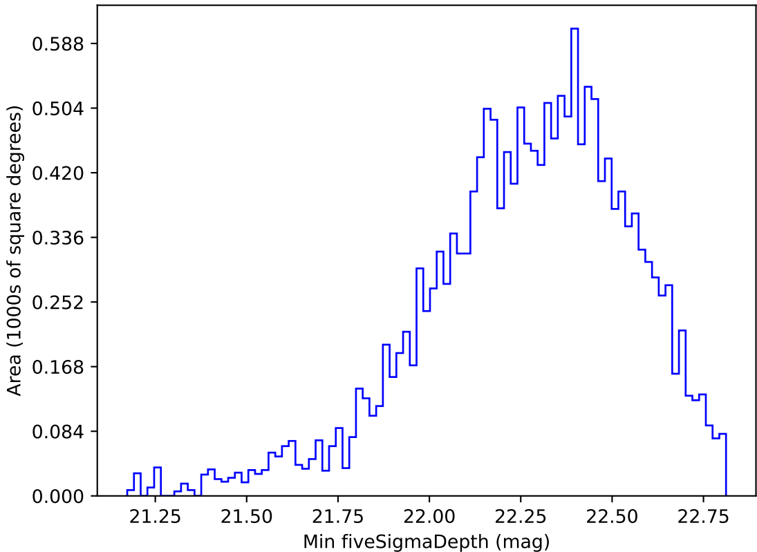
ddf_loaded_fl4_v3.4_10yrs WFD u band: Min fiveSigmaDepth
