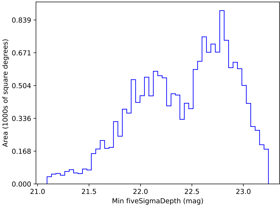
ddf_loaded_fl4_v3.4_10yrs WFD r band: Min fiveSigmaDepth
