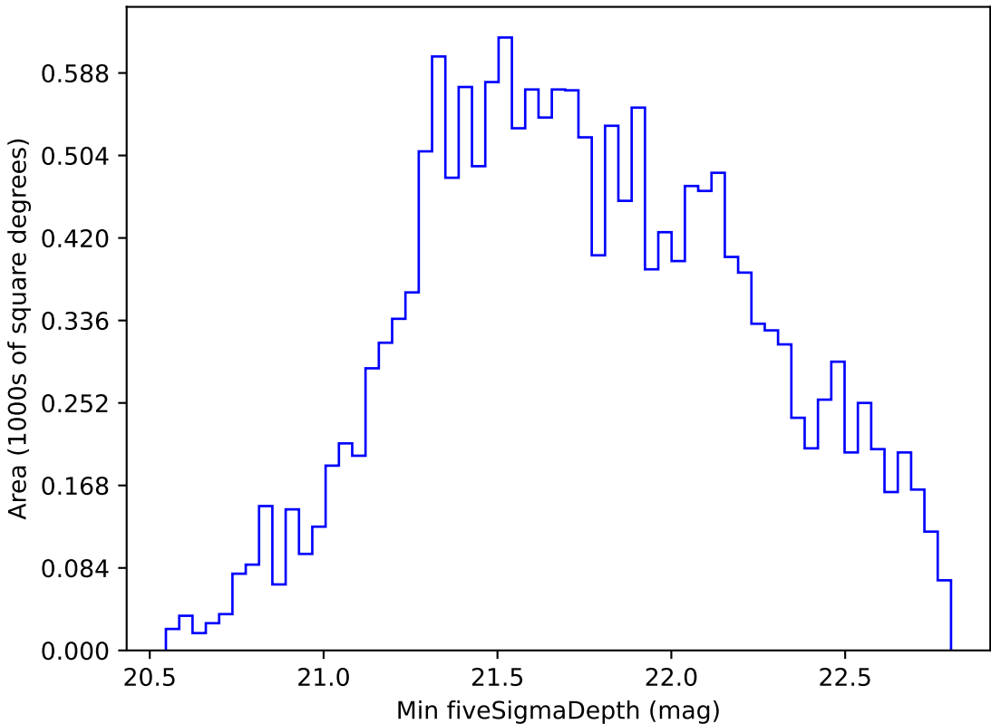
ddf_loaded_fl4_v3.4_10yrs WFD i band: Min fiveSigmaDepth
