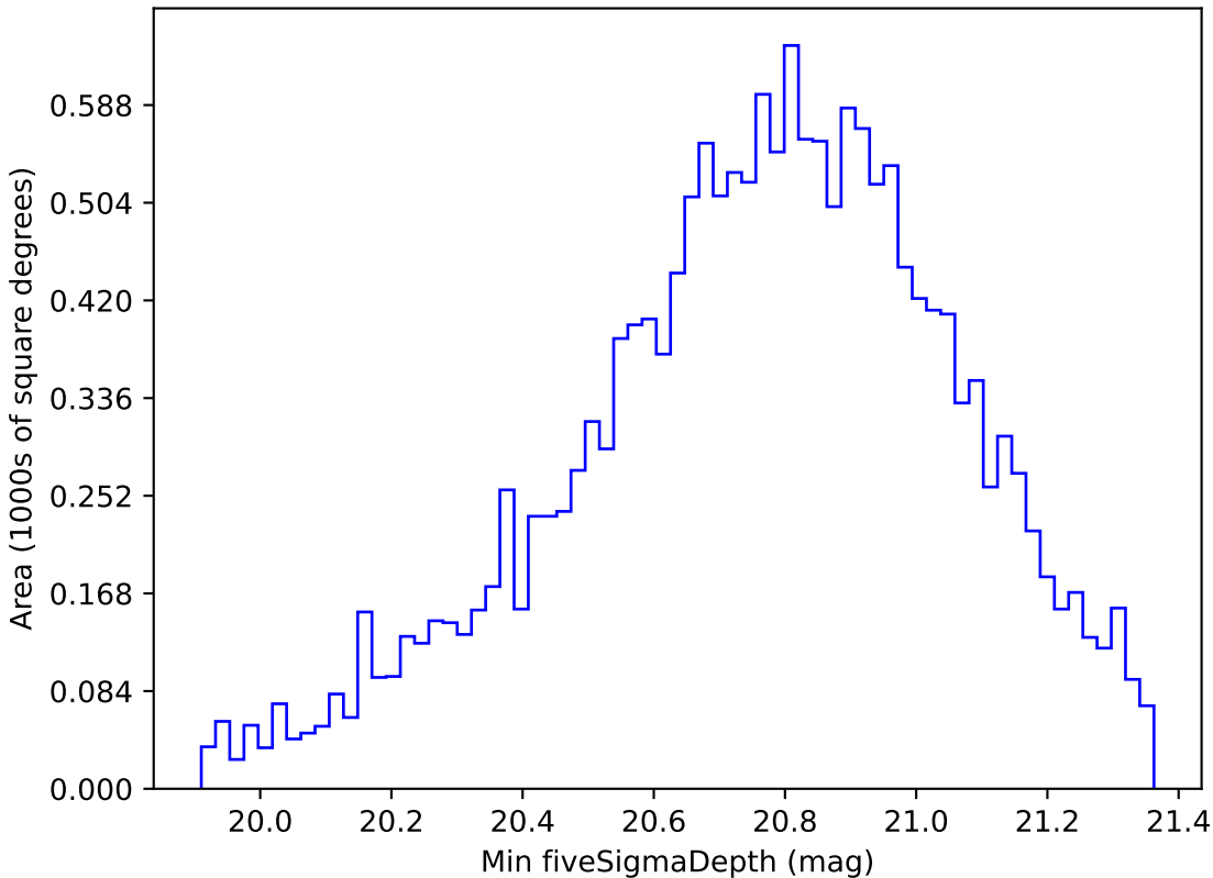
ddf_loaded_fl4_v3.4_10yrs WFD all bands: Min fiveSigmaDepth
