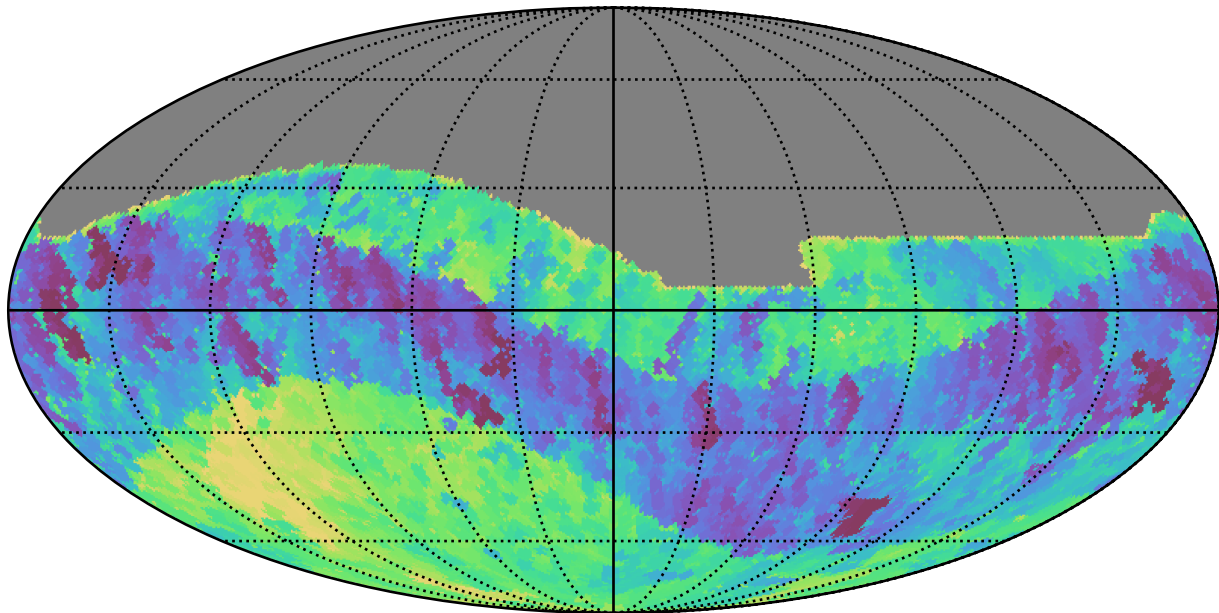
ddf_loaded_fl4_v3.4_10yrs All sky z band: Min fiveSigmaDepth
