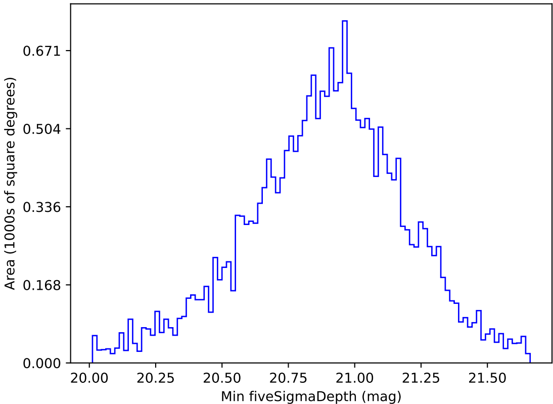
ddf_loaded_fl4_v3.4_10yrs All sky y band: Min fiveSigmaDepth
