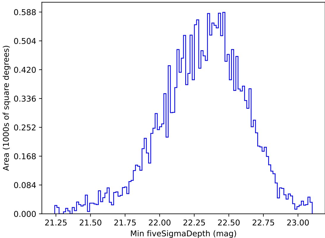
ddf_loaded_fl4_v3.4_10yrs All sky u band: Min fiveSigmaDepth
