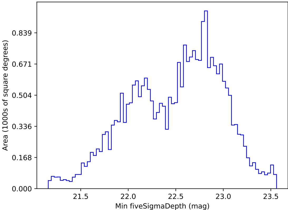
ddf_loaded_fl4_v3.4_10yrs All sky r band: Min fiveSigmaDepth
