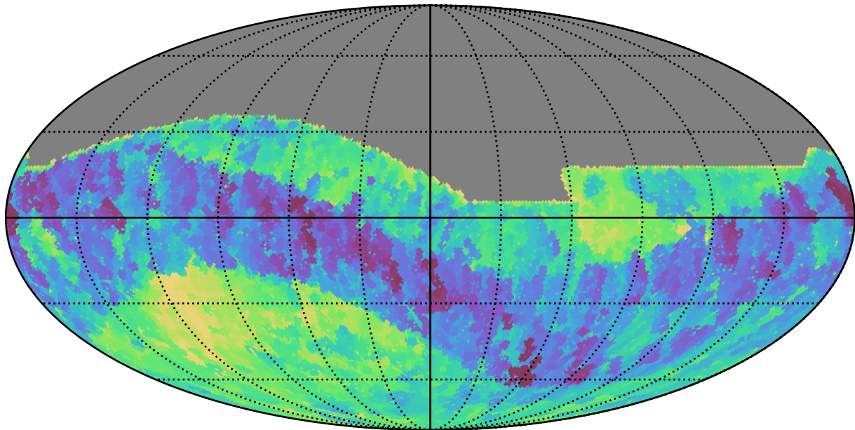
ddf_loaded_fl4_v3.4_10yrs All sky i band: Min fiveSigmaDepth
