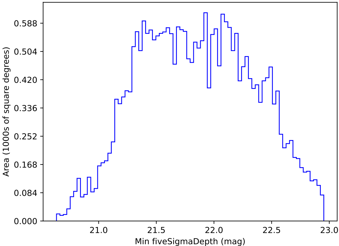
ddf_loaded_fl4_v3.4_10yrs All sky i band: Min fiveSigmaDepth
