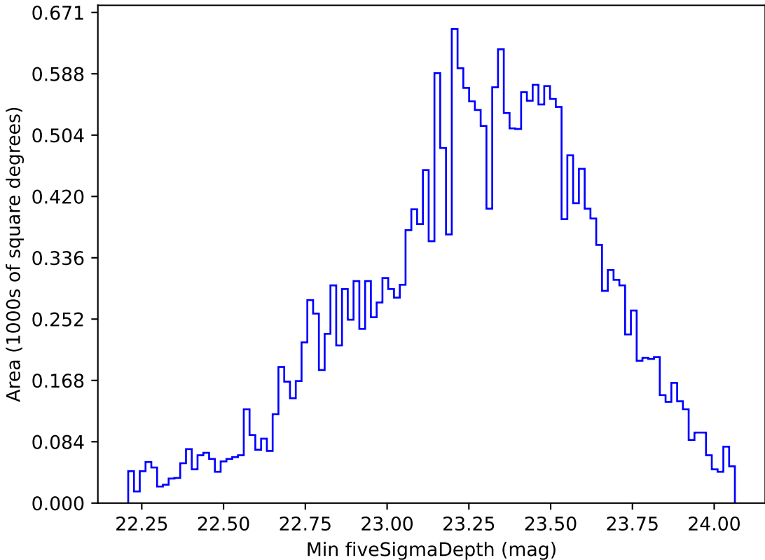
ddf_loaded_fl4_v3.4_10yrs All sky g band: Min fiveSigmaDepth
