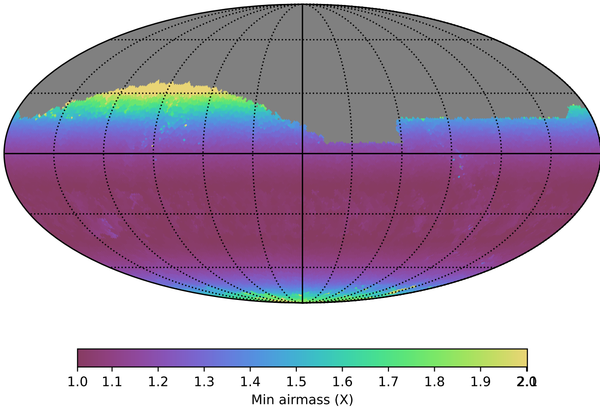
ddf_loaded_fl4_v3.4_10yrs Yr 1 z band: Min airmass
