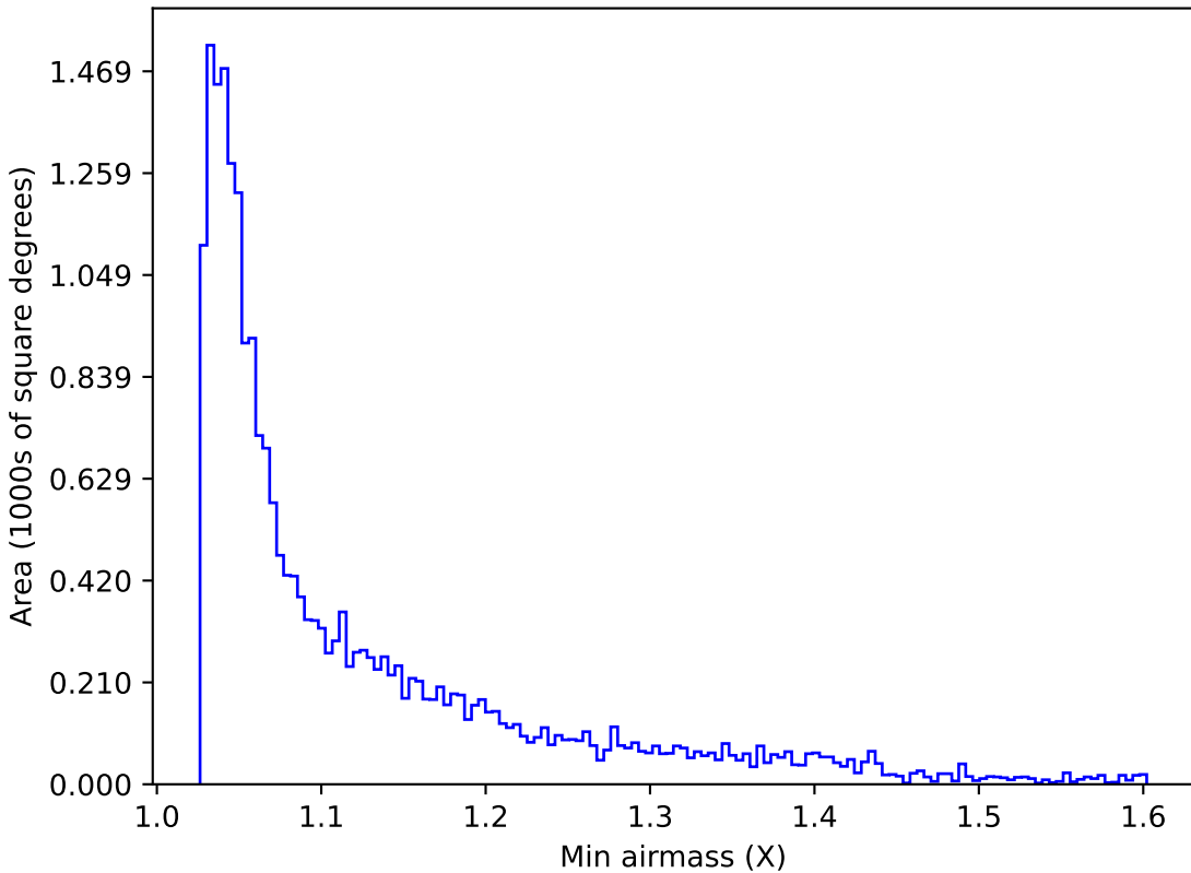
ddf_loaded_fl4_v3.4_10yrs Yr 1 y band: Min airmass
