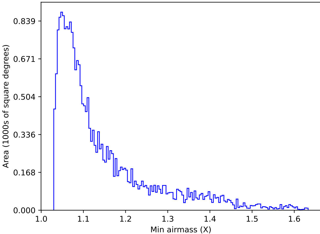
ddf_loaded_fl4_v3.4_10yrs Yr 1 u band: Min airmass
