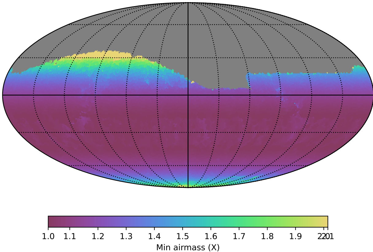
ddf_loaded_fl4_v3.4_10yrs Yr 1 r band: Min airmass
