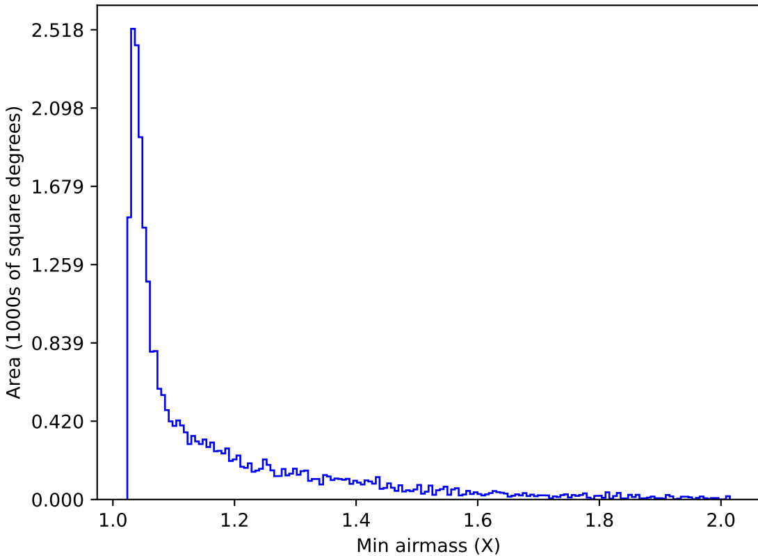
ddf_loaded_fl4_v3.4_10yrs Yr 1 r band: Min airmass
