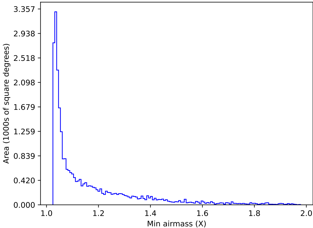
ddf_loaded_fl4_v3.4_10yrs Yr 1 i band: Min airmass
