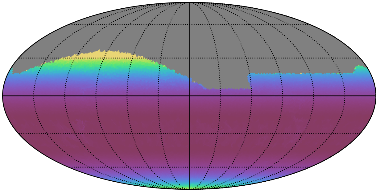
ddf_loaded_fl4_v3.4_10yrs Yr 1 all bands: Min airmass
