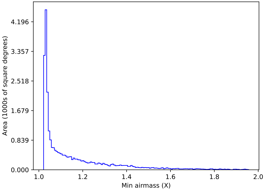
ddf_loaded_fl4_v3.4_10yrs Yr 1 all bands: Min airmass
