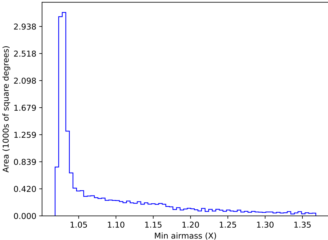
ddf_loaded_fl4_v3.4_10yrs WFD z band: Min airmass
