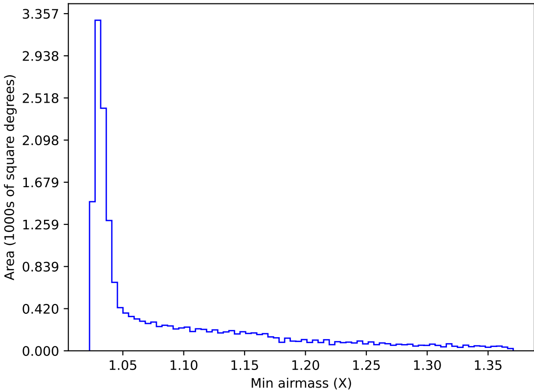
ddf_loaded_fl4_v3.4_10yrs WFD y band: Min airmass
