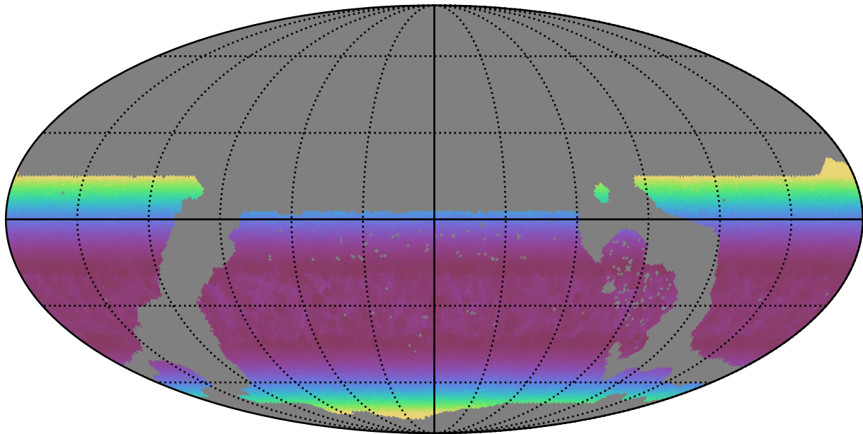
ddf_loaded_fl4_v3.4_10yrs WFD u band: Min airmass
