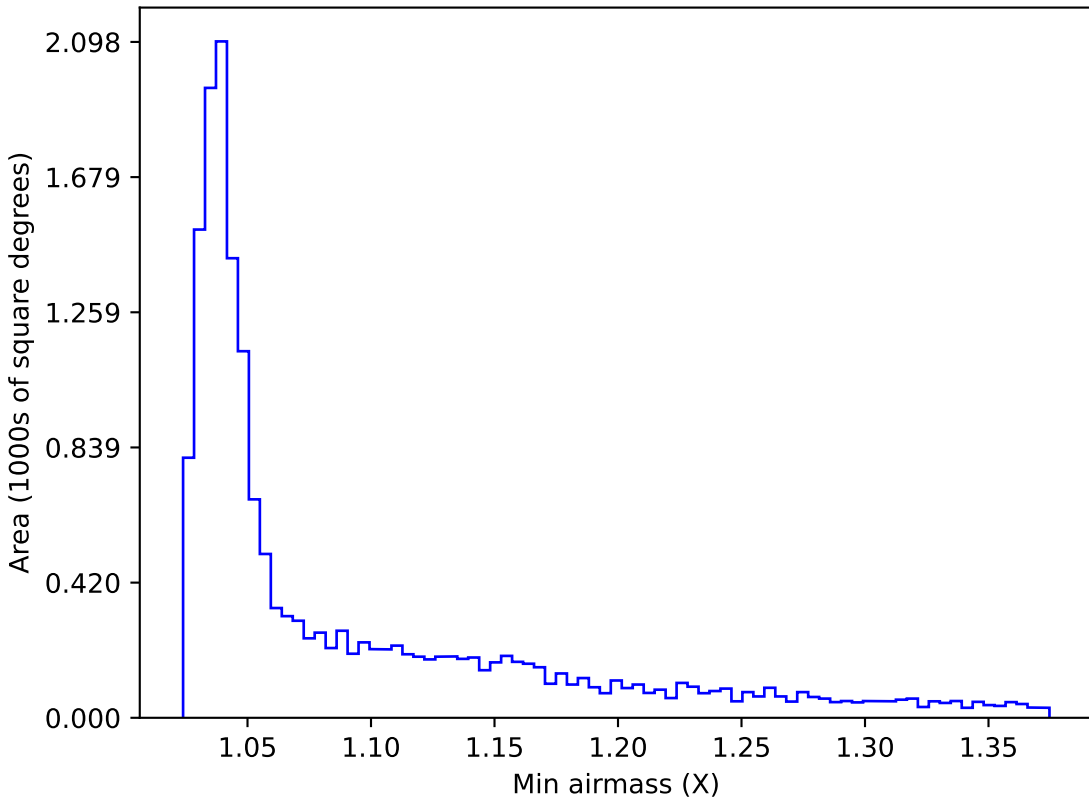
ddf_loaded_fl4_v3.4_10yrs WFD u band: Min airmass
