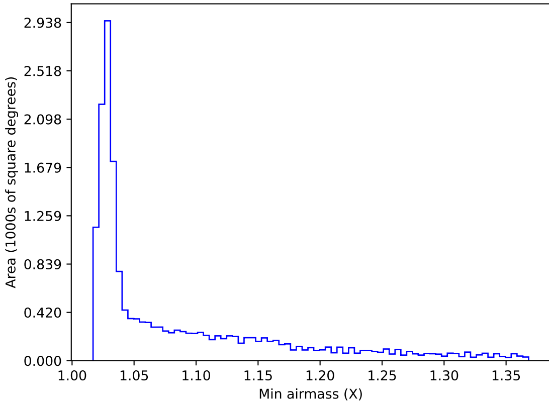
ddf_loaded_fl4_v3.4_10yrs WFD r band: Min airmass
