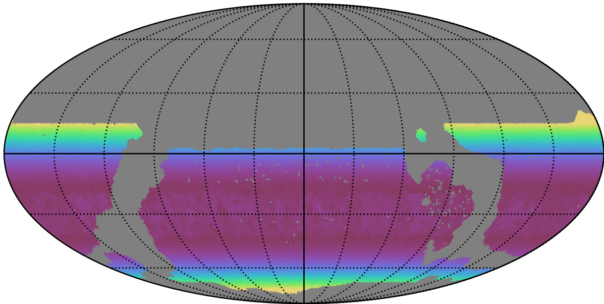
ddf_loaded_fl4_v3.4_10yrs WFD g band: Min airmass
