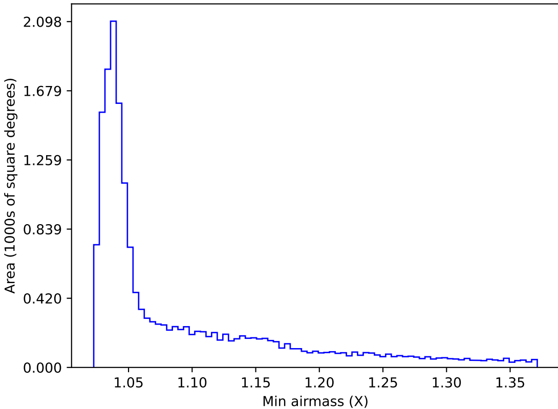
ddf_loaded_fl4_v3.4_10yrs WFD g band: Min airmass
