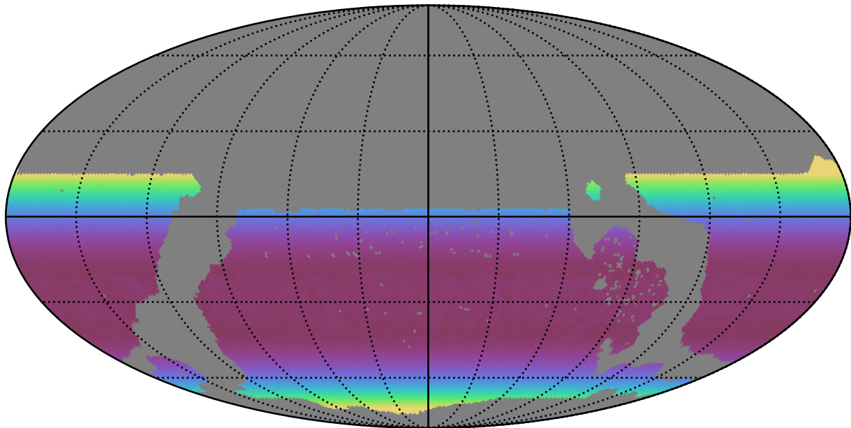
ddf_loaded_fl4_v3.4_10yrs WFD all bands: Min airmass
