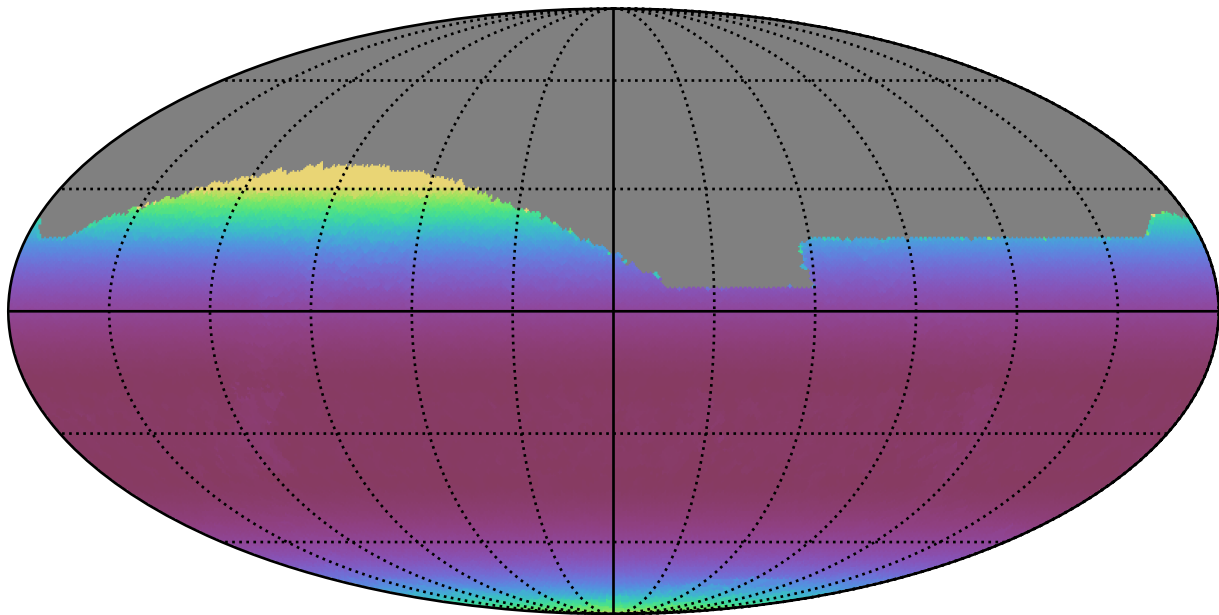
ddf_loaded_fl4_v3.4_10yrs All sky z band: Min airmass
