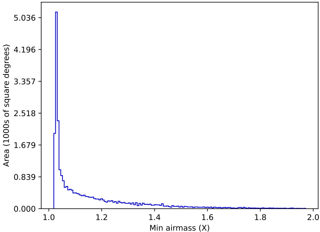
ddf_loaded_fl4_v3.4_10yrs All sky z band: Min airmass
