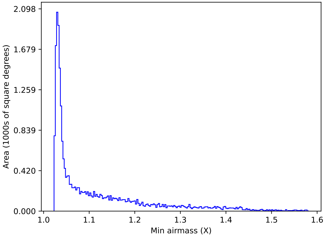
ddf_loaded_fl4_v3.4_10yrs All sky y band: Min airmass
