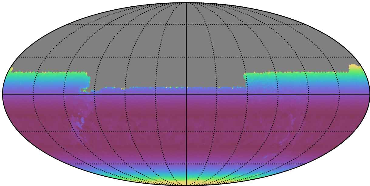
ddf_loaded_fl4_v3.4_10yrs All sky u band: Min airmass
