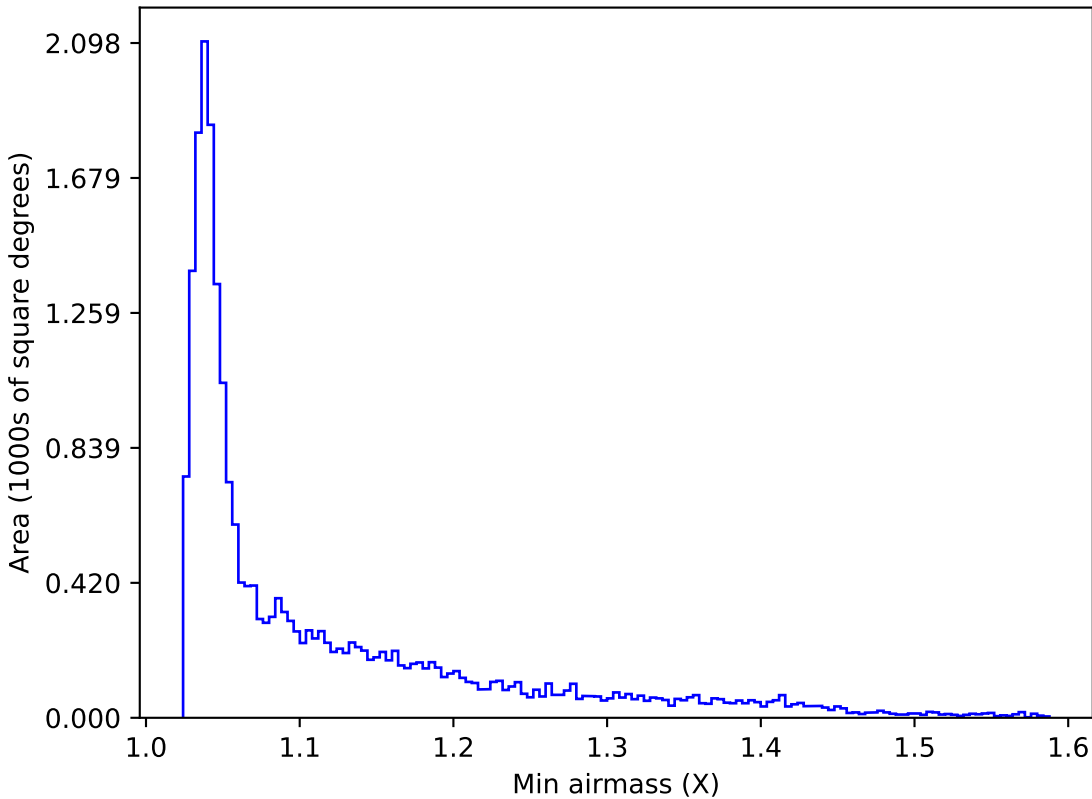
ddf_loaded_fl4_v3.4_10yrs All sky u band: Min airmass
