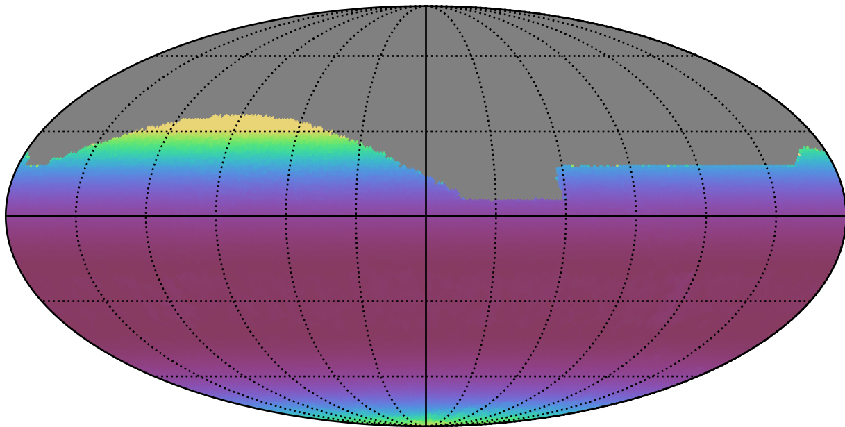
ddf_loaded_fl4_v3.4_10yrs All sky r band: Min airmass
