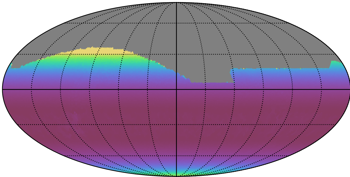
ddf_loaded_fl4_v3.4_10yrs All sky i band: Min airmass
