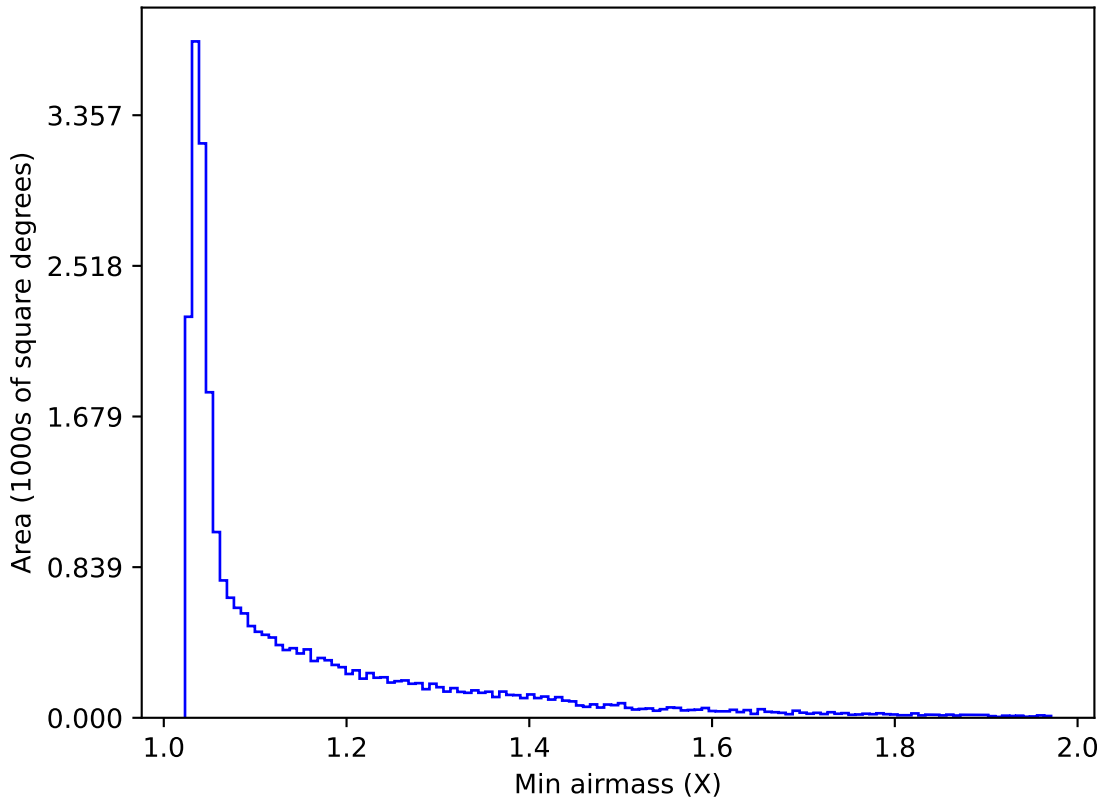
ddf_loaded_fl4_v3.4_10yrs All sky g band: Min airmass
