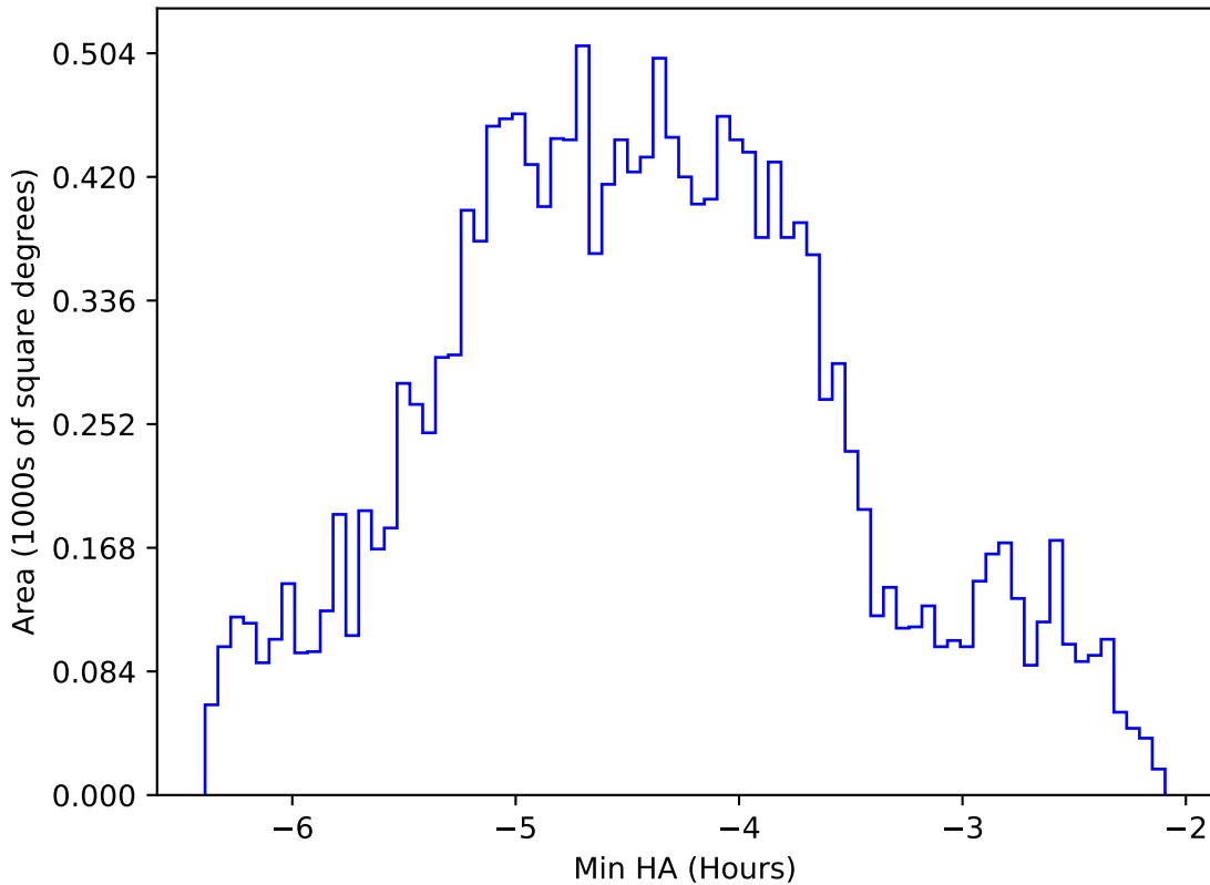
ddf_loaded_fl4_v3.4_10yrs WFD z band: Min HA
