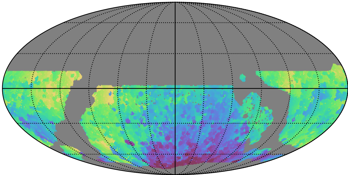
ddf_loaded_fl4_v3.4_10yrs WFD y band: Min HA
