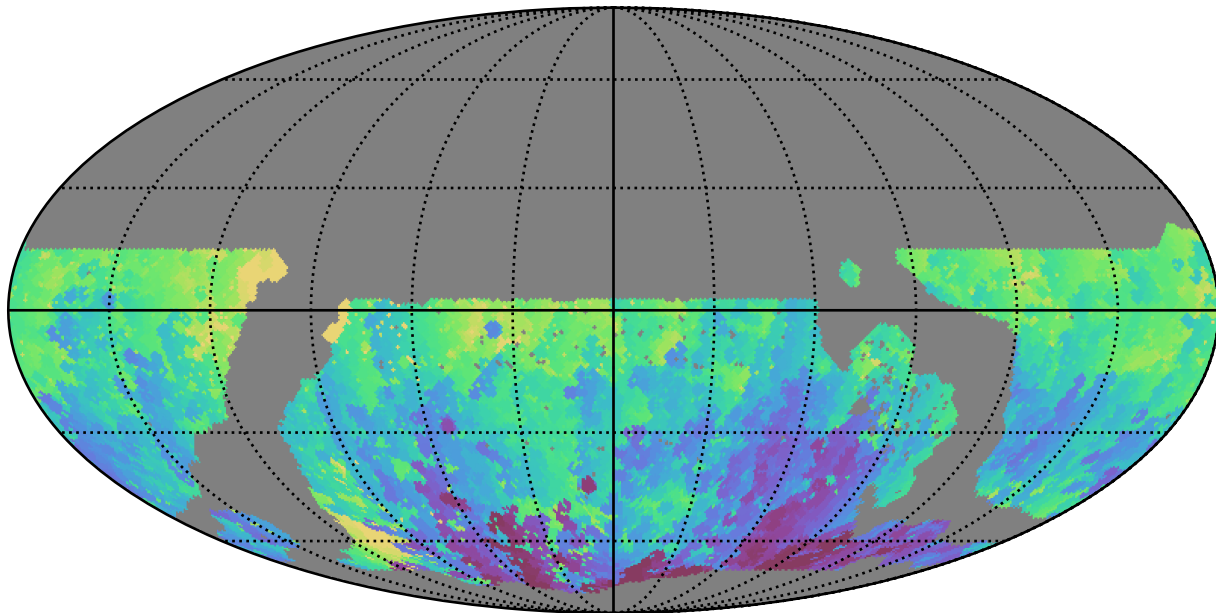
ddf_loaded_fl4_v3.4_10yrs WFD u band: Min HA
