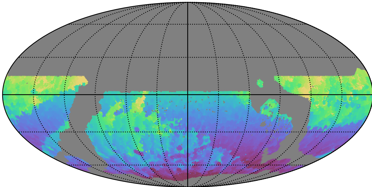
ddf_loaded_fl4_v3.4_10yrs WFD r band: Min HA
