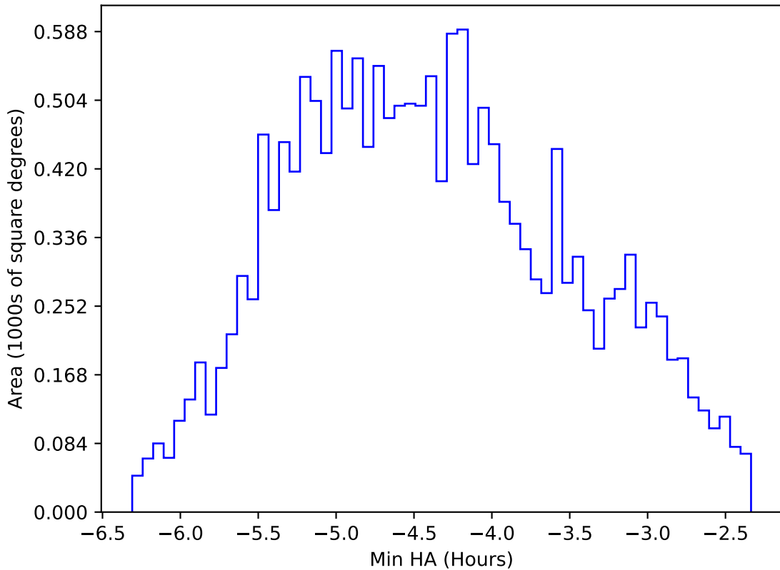
ddf_loaded_fl4_v3.4_10yrs WFD r band: Min HA
