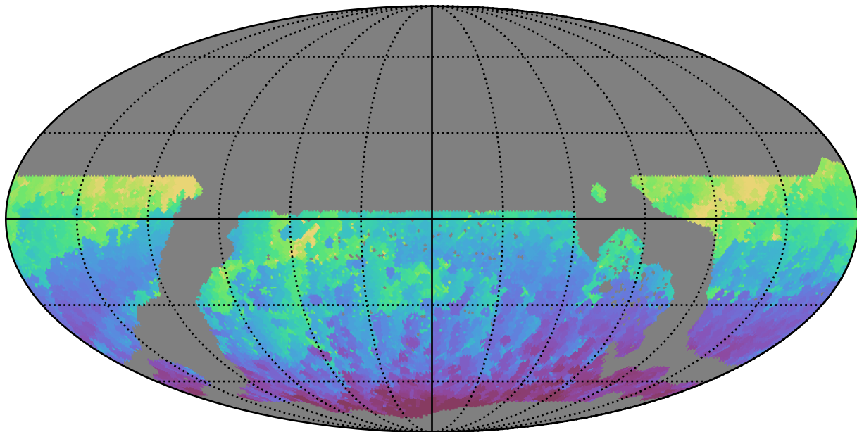
ddf_loaded_fl4_v3.4_10yrs WFD i band: Min HA
