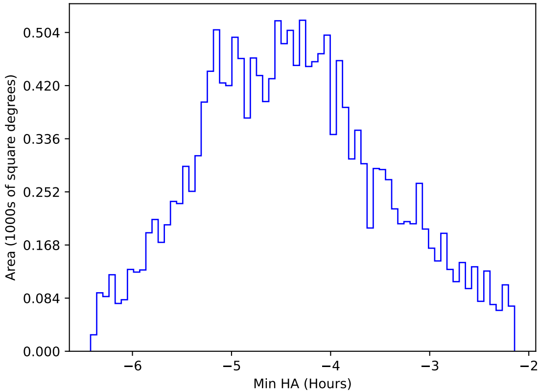
ddf_loaded_fl4_v3.4_10yrs WFD i band: Min HA
