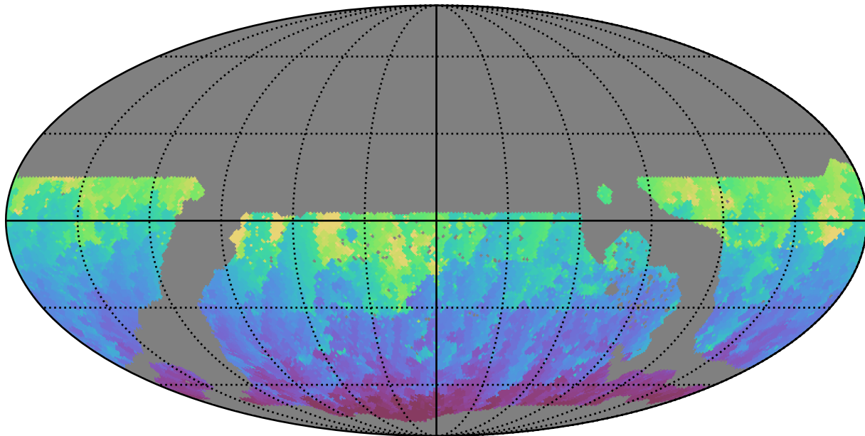
ddf_loaded_fl4_v3.4_10yrs WFD g band: Min HA
