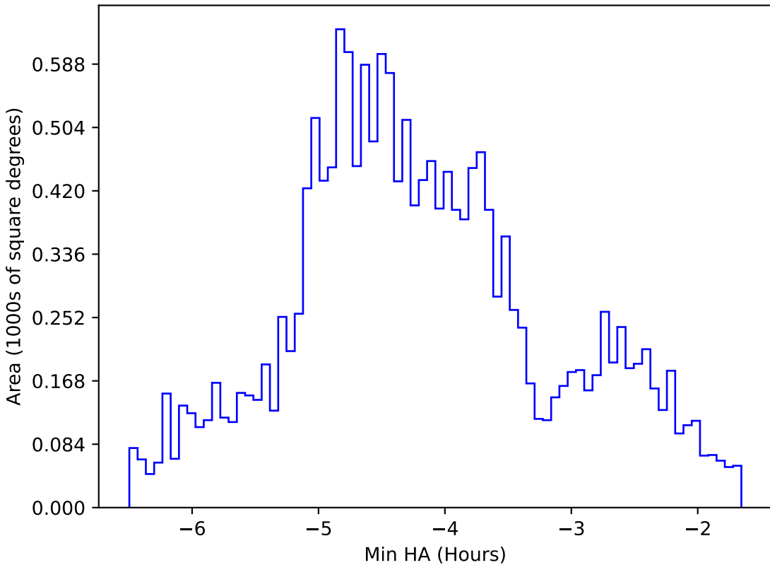
ddf_loaded_fl4_v3.4_10yrs WFD g band: Min HA
