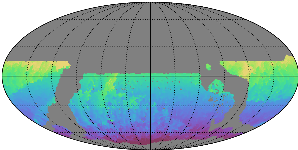
ddf_loaded_fl4_v3.4_10yrs WFD all bands: Min HA
